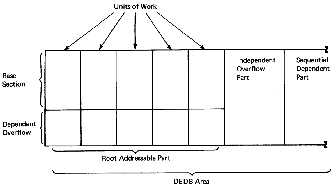
Figure 6-4. DEDB Units-of-Work
