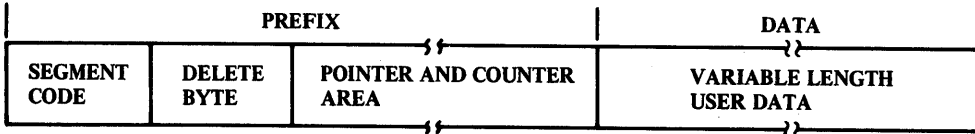
Figure 4-1. Segment Formats
