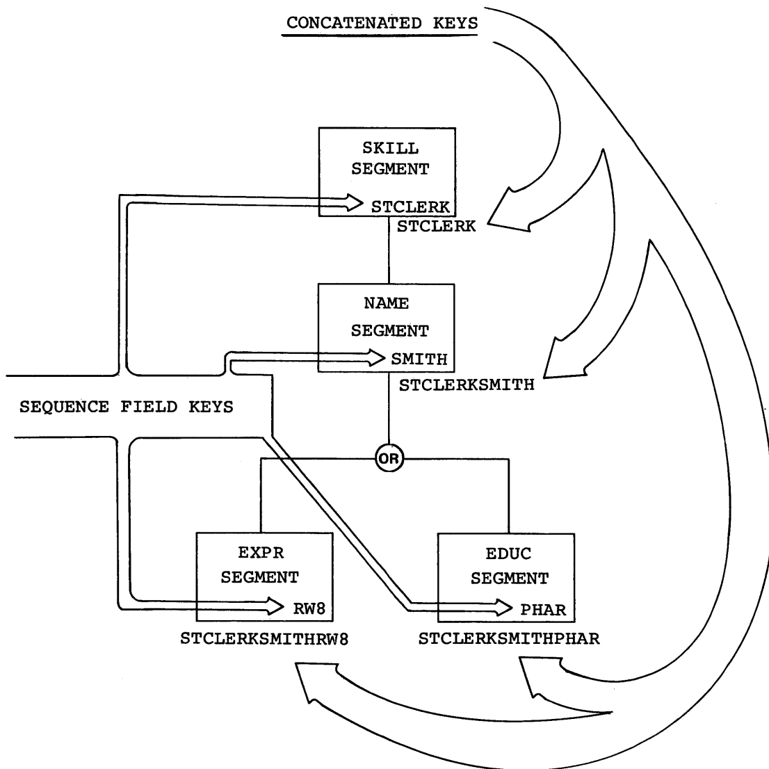
Figure 4-3. Concatenated Keys
