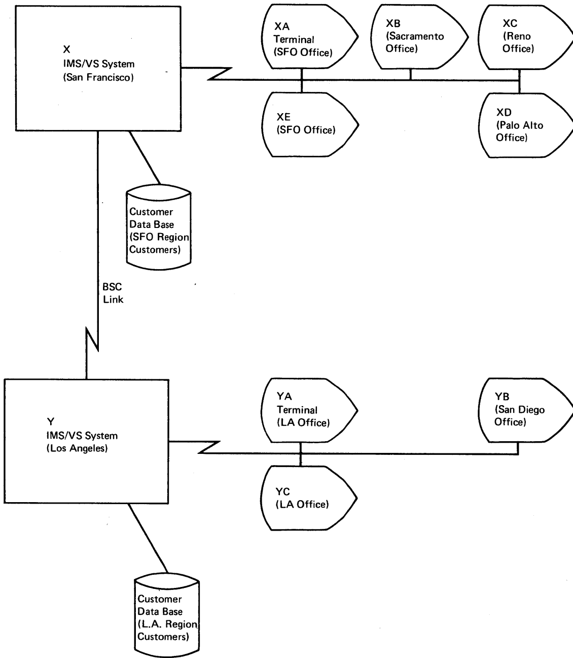
Figure 5-12. Horizontal Partitioning
