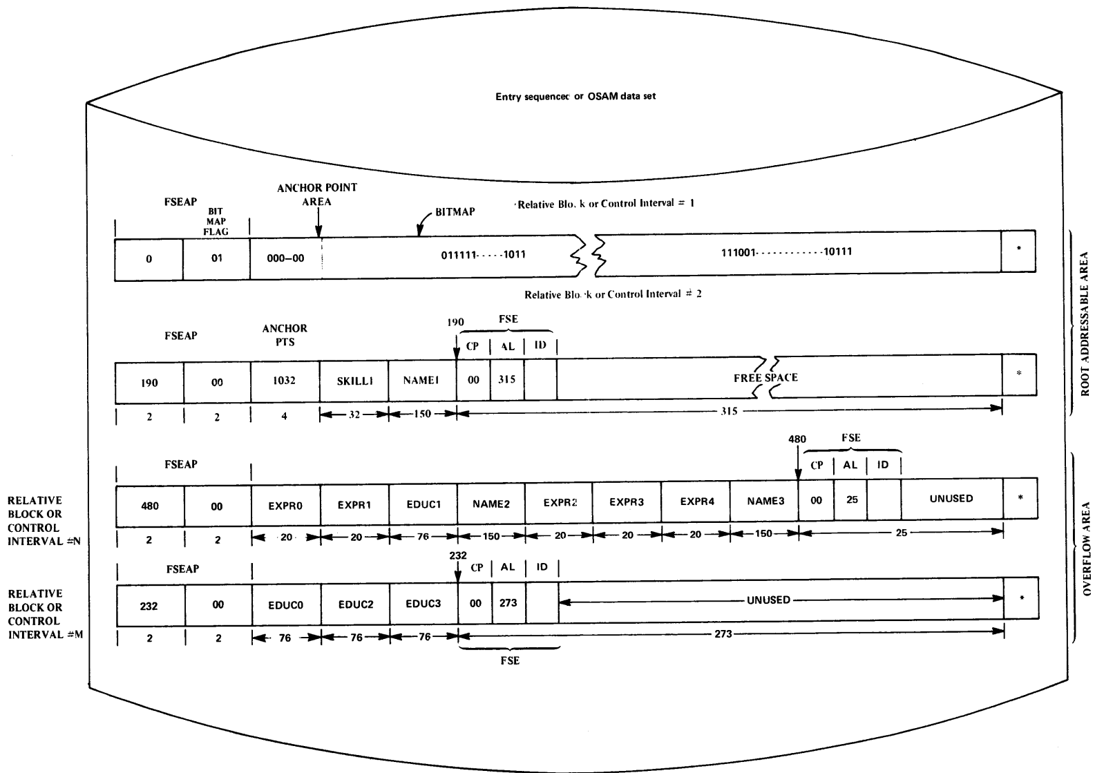
Figure 4-22.
