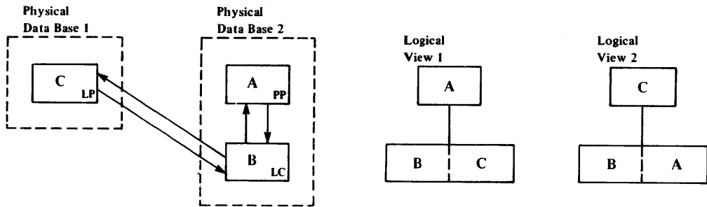
Figure 4-33. Replace Rules
