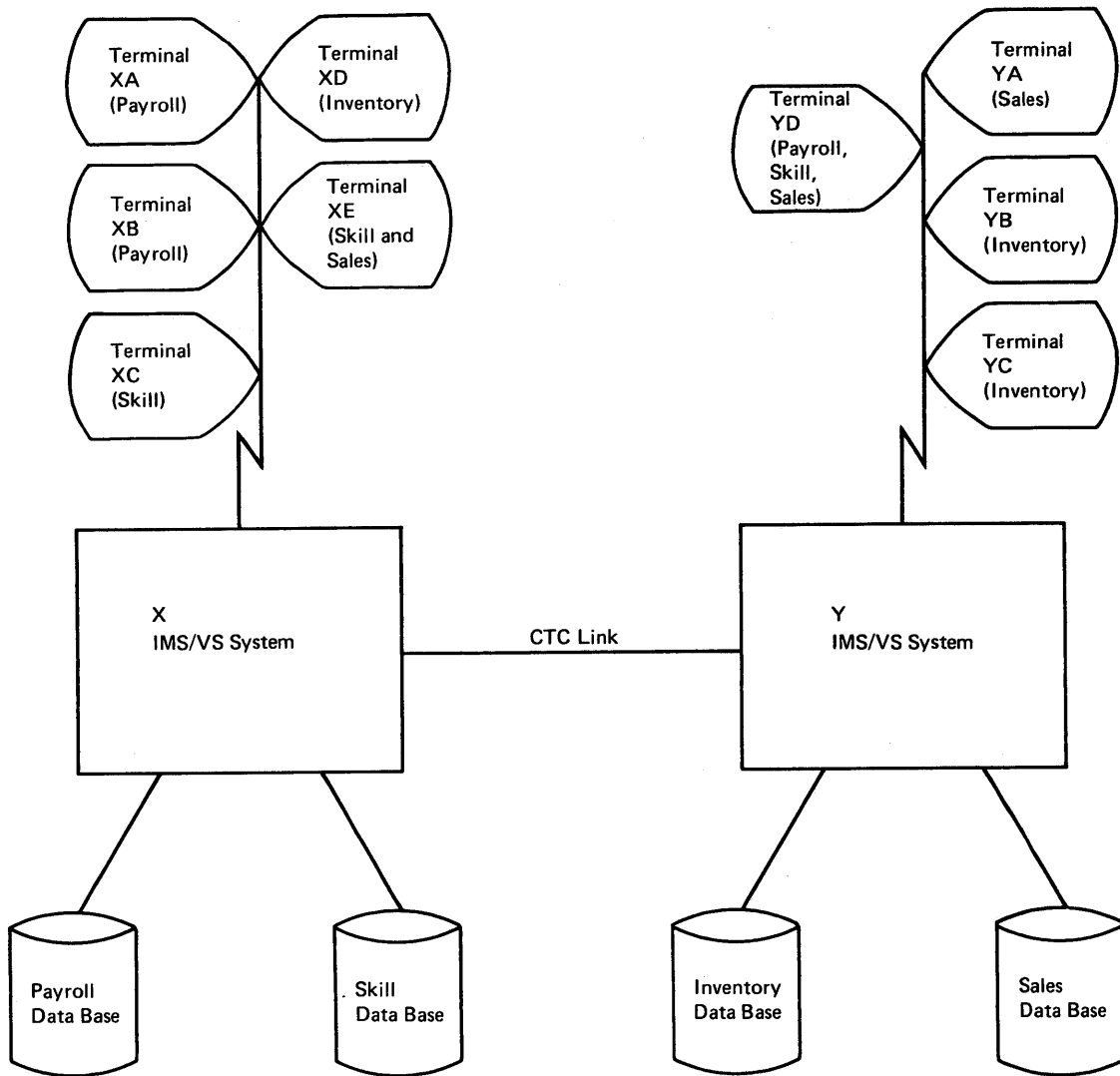
Figure 5-13. Vertical Partitioning
