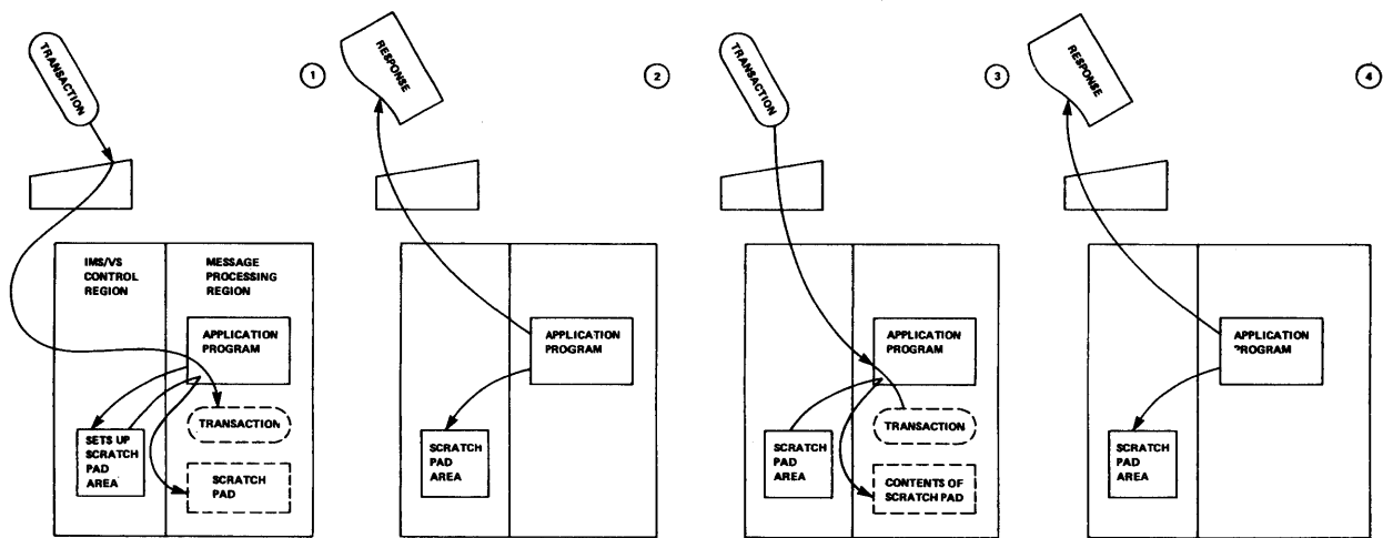
Figure 3-15. Conversational Program
