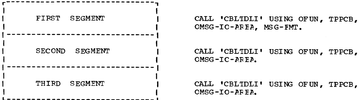
Figure 3-11. Three-Segment Message
