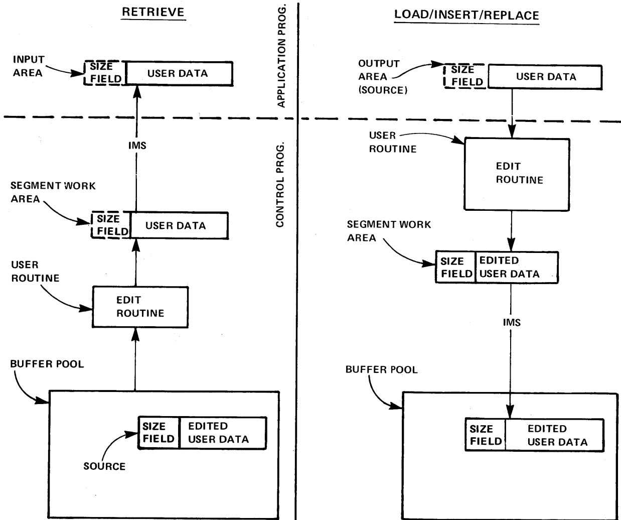
Figure 4-44. Segment Edit/Compression
